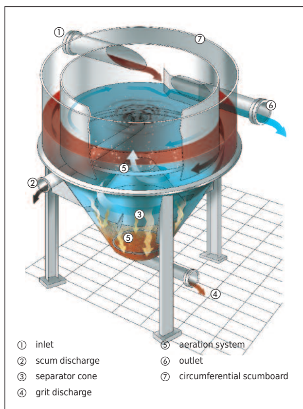
Flow diagram of a HUBER Circular Grit Trap HRSF
